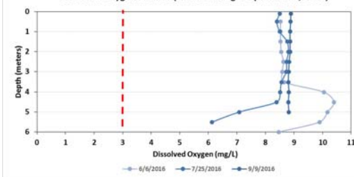
Figure 6. Lake Ivanhoe - Site 2 Ivanhoe Dissolved Oxygen Profiles (June 6 through Septmeber 9, 2016)
